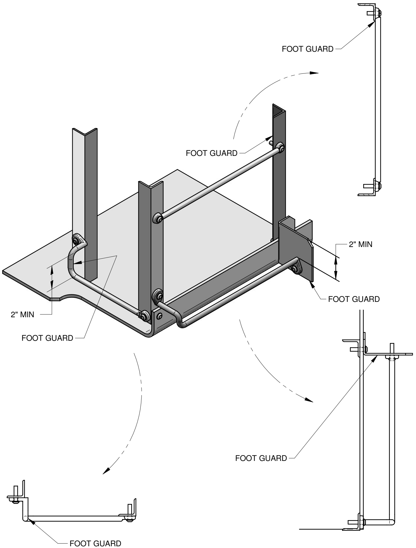
Fig. 2 Foot guards
