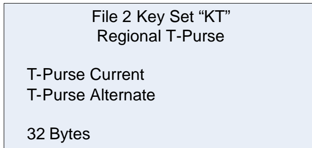
Diagram 3—File 2 Structure
